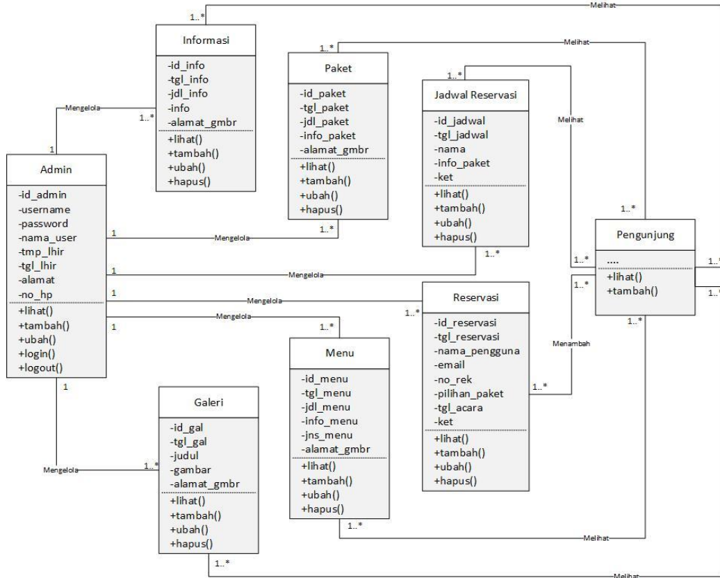
Gambar 4.4 Class Diagram [7]
