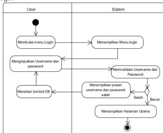
Gambar Diagram Activity Login
